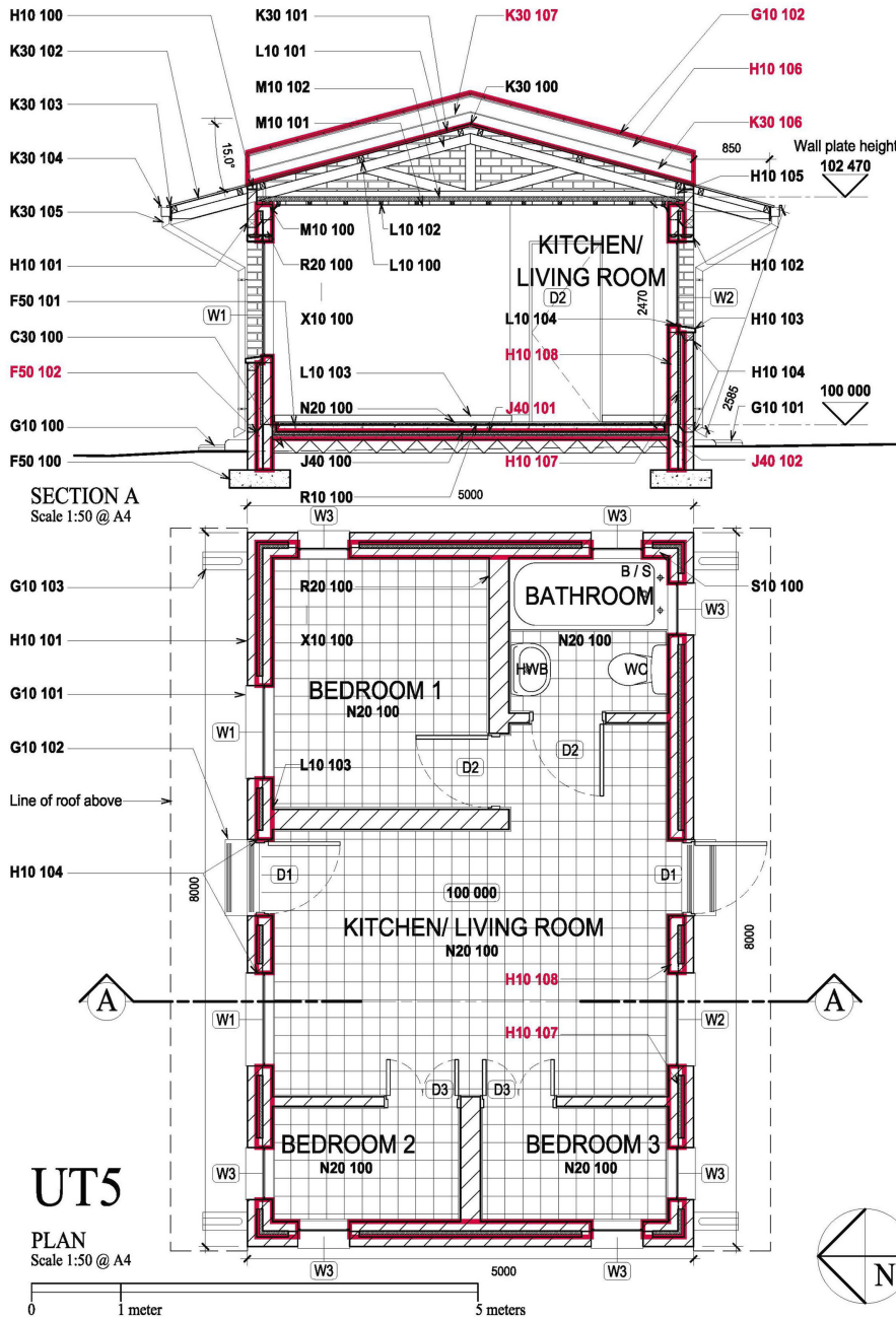
Figure 8. Unit Type 5 (UT5) architectural drawings
