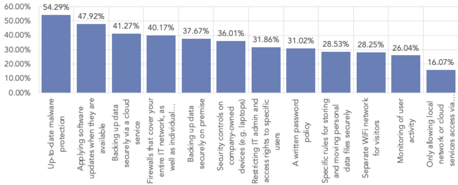
Figure 14. Ctrl1 : Implemented rules and controls
