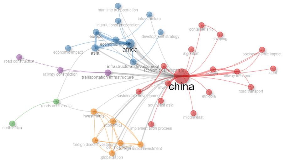
Figure 4. Co-occurrence network
