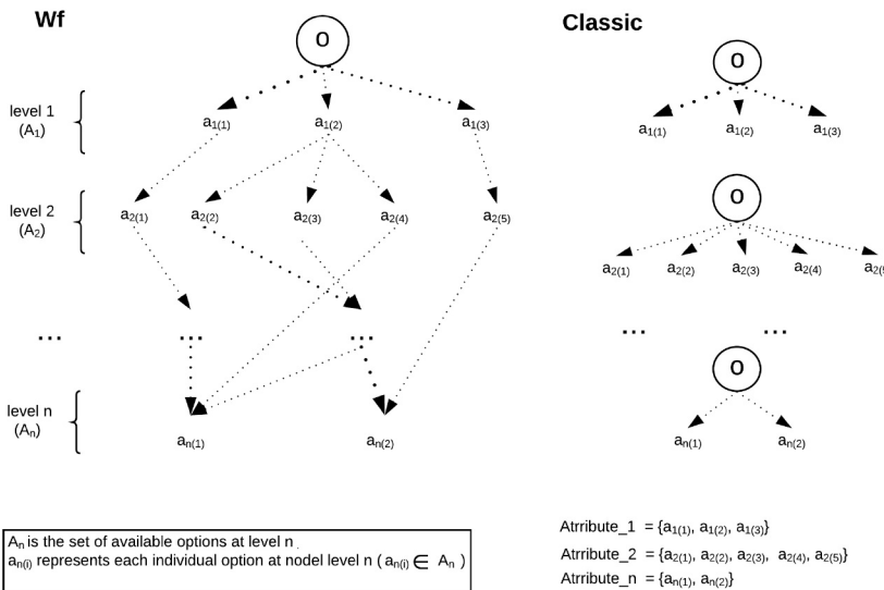
Figure 7. Graph representation of an example classification workflow W_f vs the corresponding classic way of looking at the classification with multiple questions
